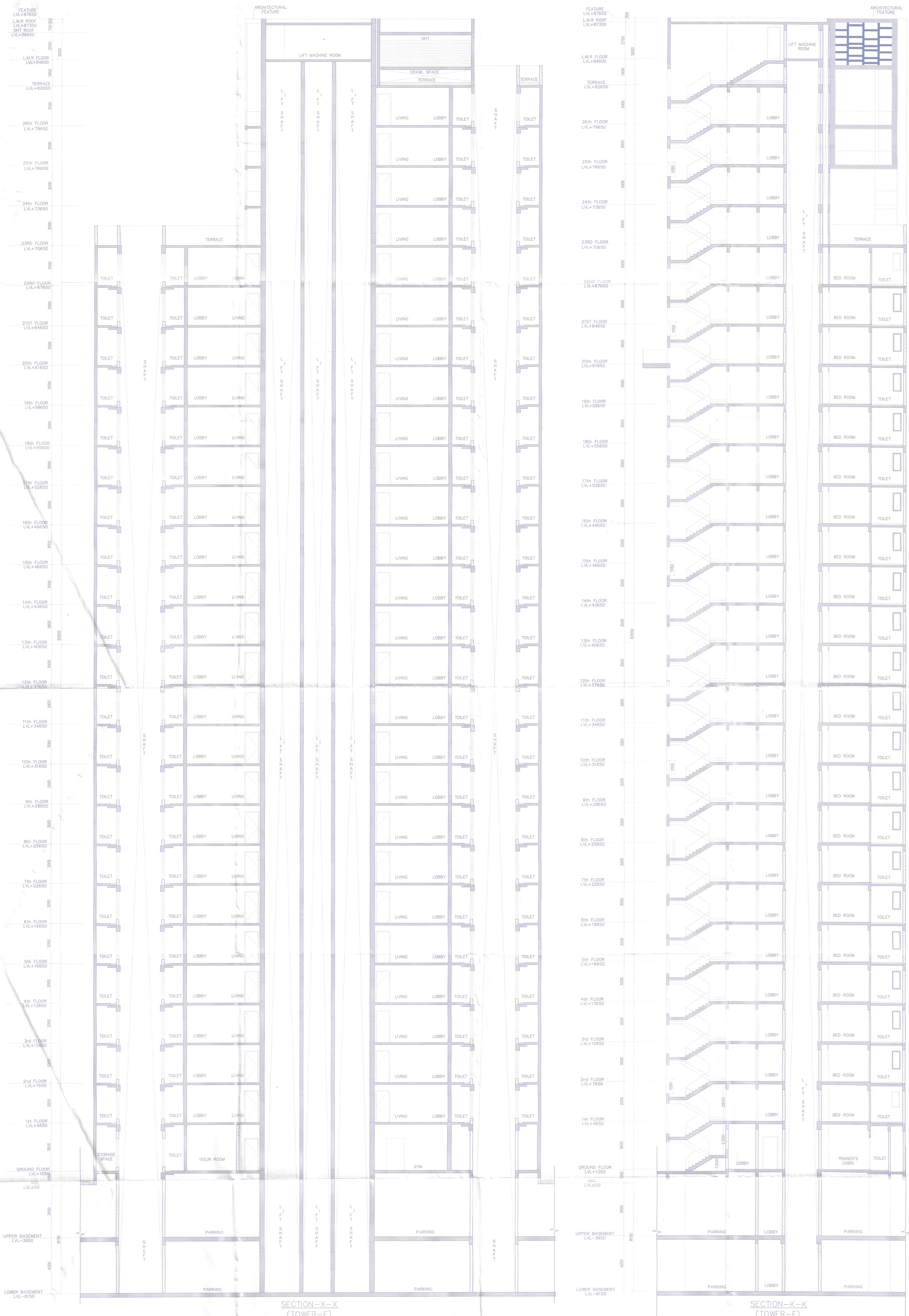
SECTION-X-X (TOWER-F)
